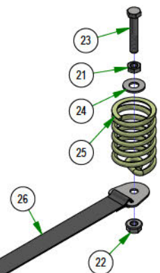
034-8045-22 2022 Mav/HD Seat Spring Assembly with Strap
