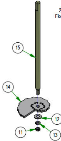
028-0070-17 ZT Deck Height Bar Assembly
