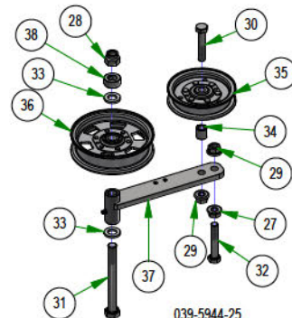
039-5944-25 Pump Idler Bracket Assembly
