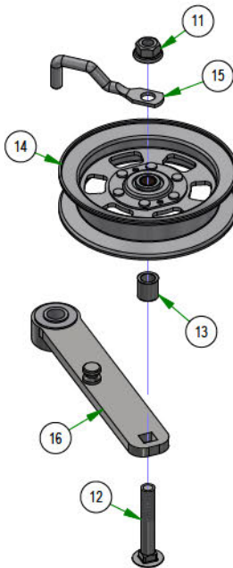
039-6945-26 Marenick HD & Down Deck Idler Assembly
