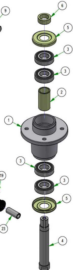
037-4000-00 Outlaw Spindle Assembly
