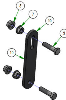
039-2127-17 Deck Hanger Assembly
