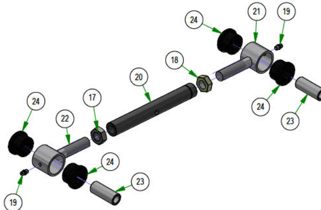
048-6000-00 2018 Maverick Tumbuckle (Top Link)
