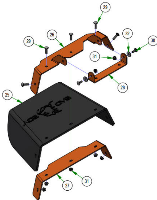
210-6025-01 2026 5in Sloped Deck Rubber Chute Assembly
