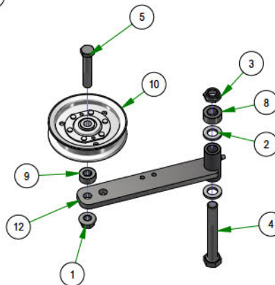
039-6945-03 REBEL TRANSAXLE IDLER ASSEMBLY
