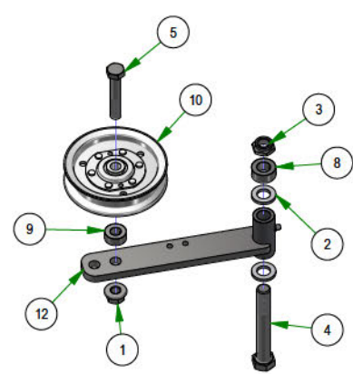
039-6945-RX REBEL X TRANSAXLE IDLER ASSEMBLY
