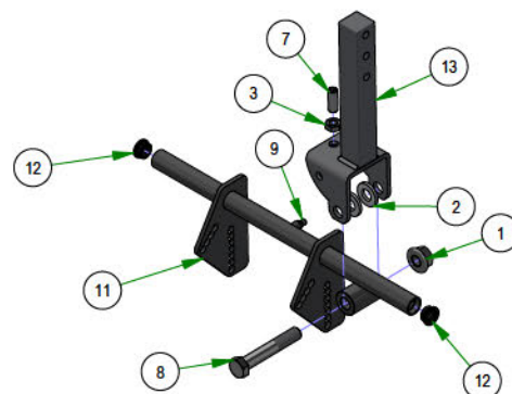
031-0031-24 LH DRIVE PIVOT ASSEMBLY
