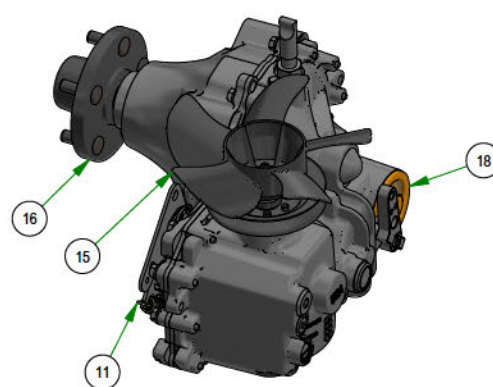
050-7000-00 & 050-7001-00 REBEL X 5400 TRANSAXLE PARTS
