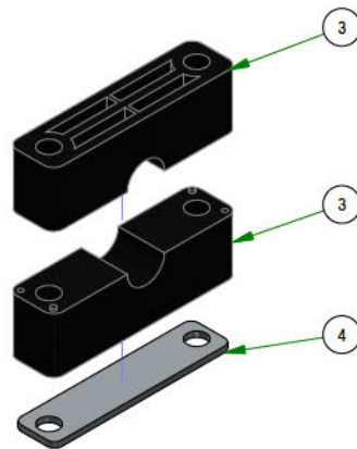
017-9075-00 PILLOW BLOCK ASSEMBLY
