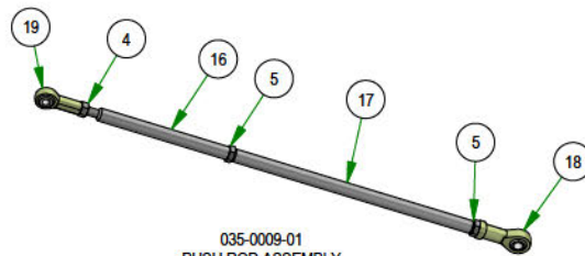
035-0009-01 PUSH ROD ASSEMBLY
