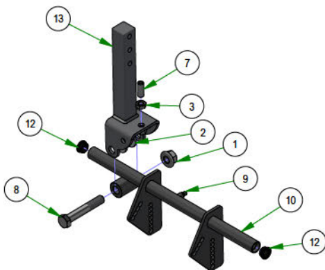
031-0030-24 RH DRIVE PIVOT ASSEMBLY
