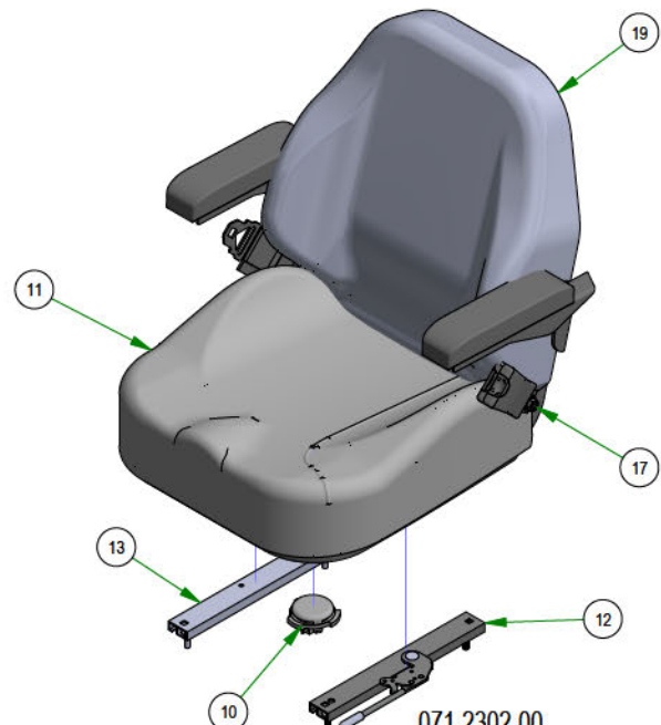
071-2302-00 SEAT ASSEMBLY
