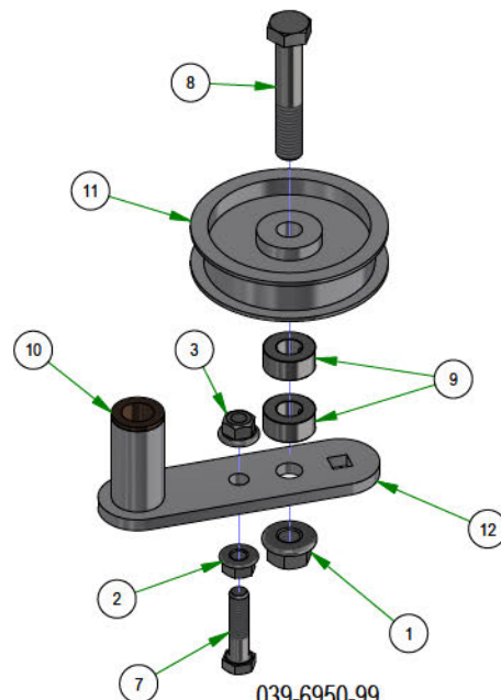
039-6950-99 RH BELT TENSIONER ASSEMBLY
