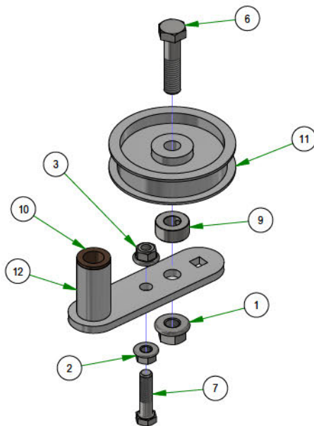
039-6950-98 LH BELT TENSIONER ASSEMBLY
