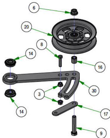
039-6946-17 DECK IDLER ASSEMBLY
