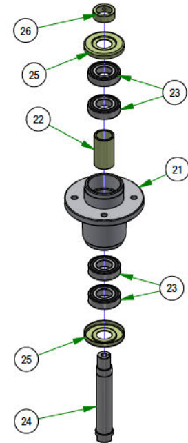
037-4000-00 DECK SPINDLE ASSEMBLY
