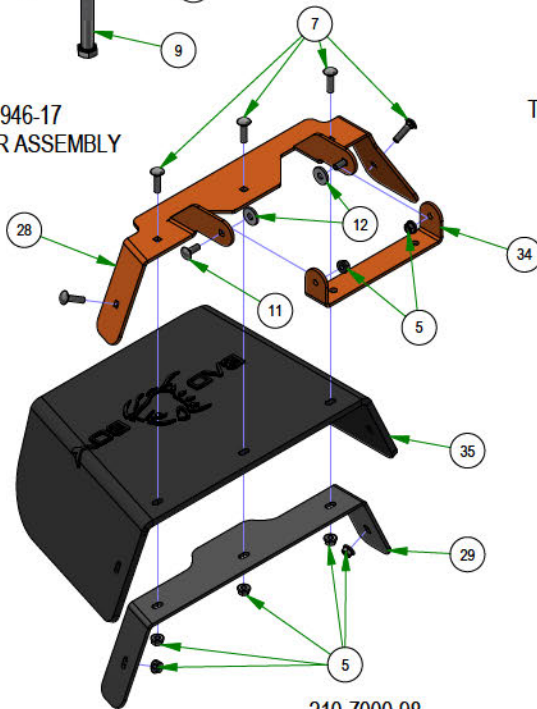
210-7000-98 CHUTE ASSEMBLY
