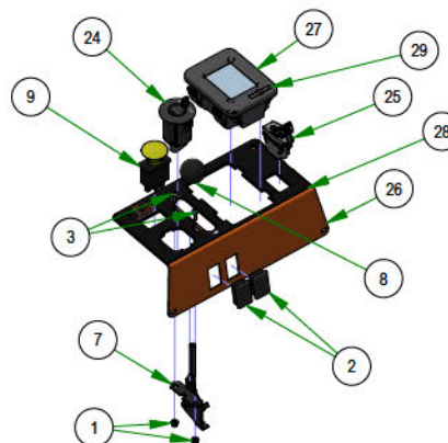
079-3482-19 CONTROL PANEL ASSEMBLY
