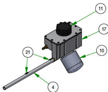
067-8053-18 LH HYDRO TANK ASSEMBLY
