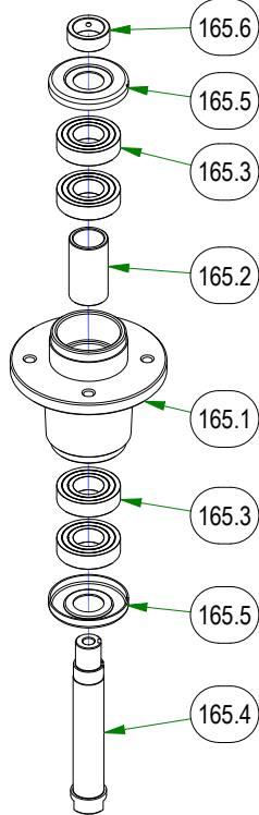
037-4000-00 SPINDLE ASSEMBLY
