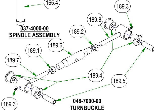
039-2125-17 DECK HANGER
